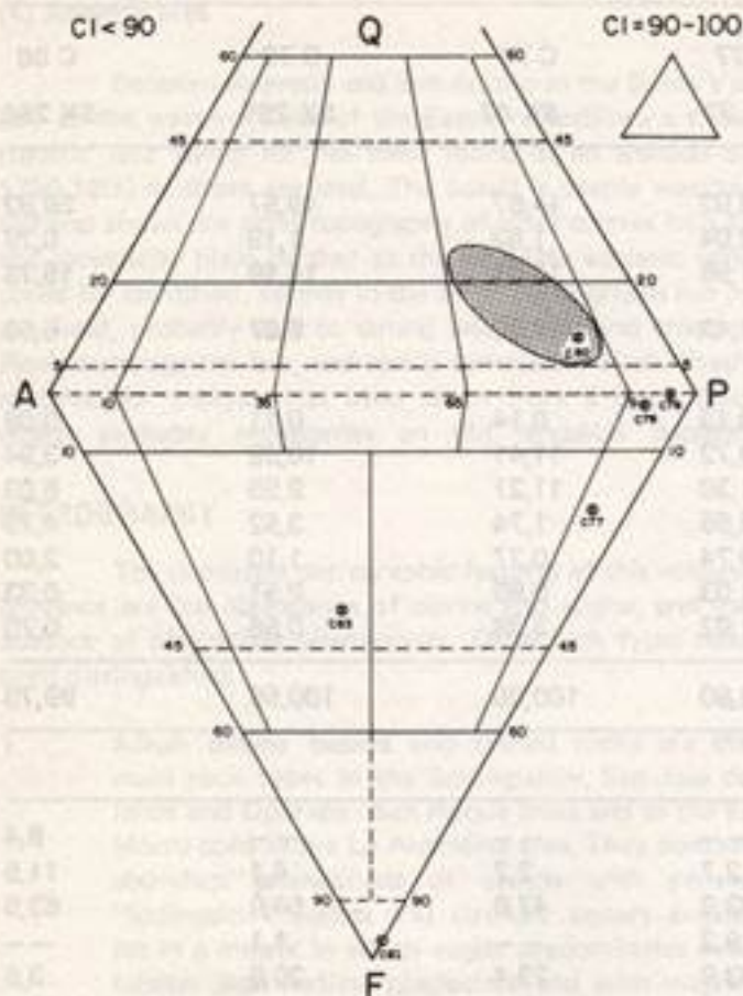
FIG. 2. Strecheisen plot of Rittmann norms of analysed sample. Dotted field represents compositional range of Cenozoic volcanics of the southern and central Colombian Andes.
